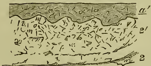
Fig. 12.—Section on Sepham Farm, on the lower slope of the Chalk hills.
